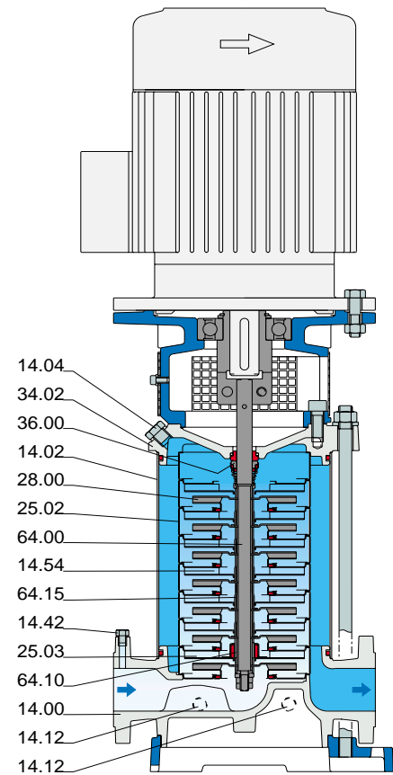
MXV 50-16, 65-32, 80-48
